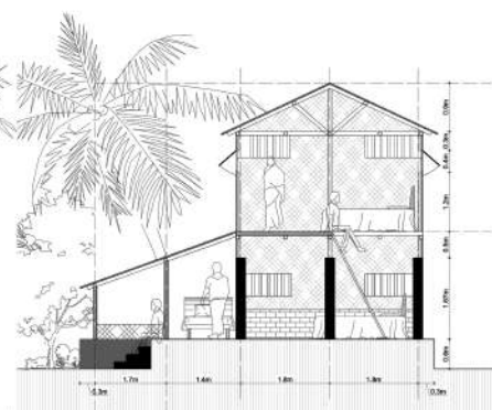
SECTION BLOW UP SCALE- 1:100
