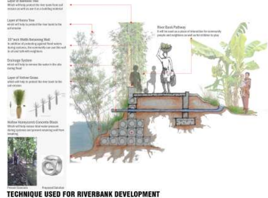
TECHNIQUE USED FOR RIVERBANK DEVELOPMENT
