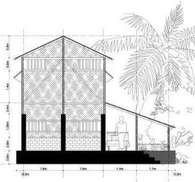
ELEVATION BLOW UP SCALE- 1:100
